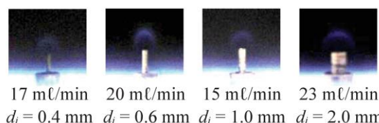
Fig.3 Premixed microflame
