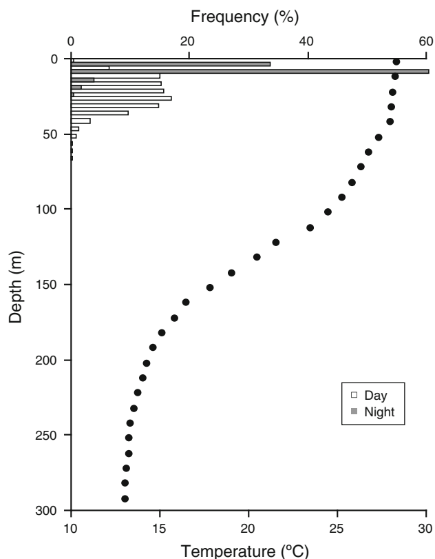
Fig. 4 Daytime ( open ) and nighttime ( solid ) depth distribution of YT11 and vertical profile of ambient water temperature. The juvenile was swimming in significantly deeper waters during the daytime. A thermocline existed from 120 to 160 m where the water temperature declined from 24°C to 17°C
