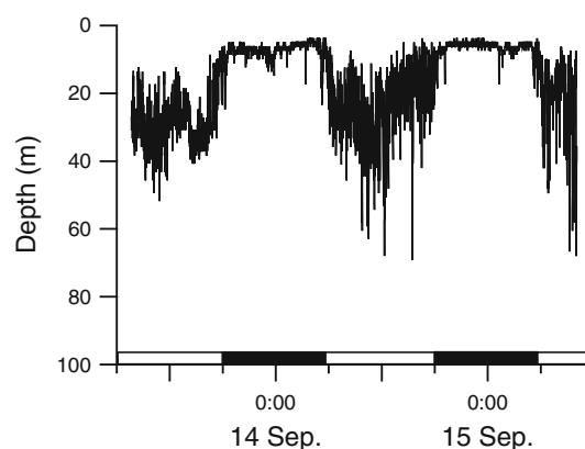
Fig. 3 Time-series data of swimming depth of YT11 on P7. The juvenile swam within a limited shallow range during nighttime (indicated by a horizontal black bar) and dived to deeper waters during daytime (white bar)
